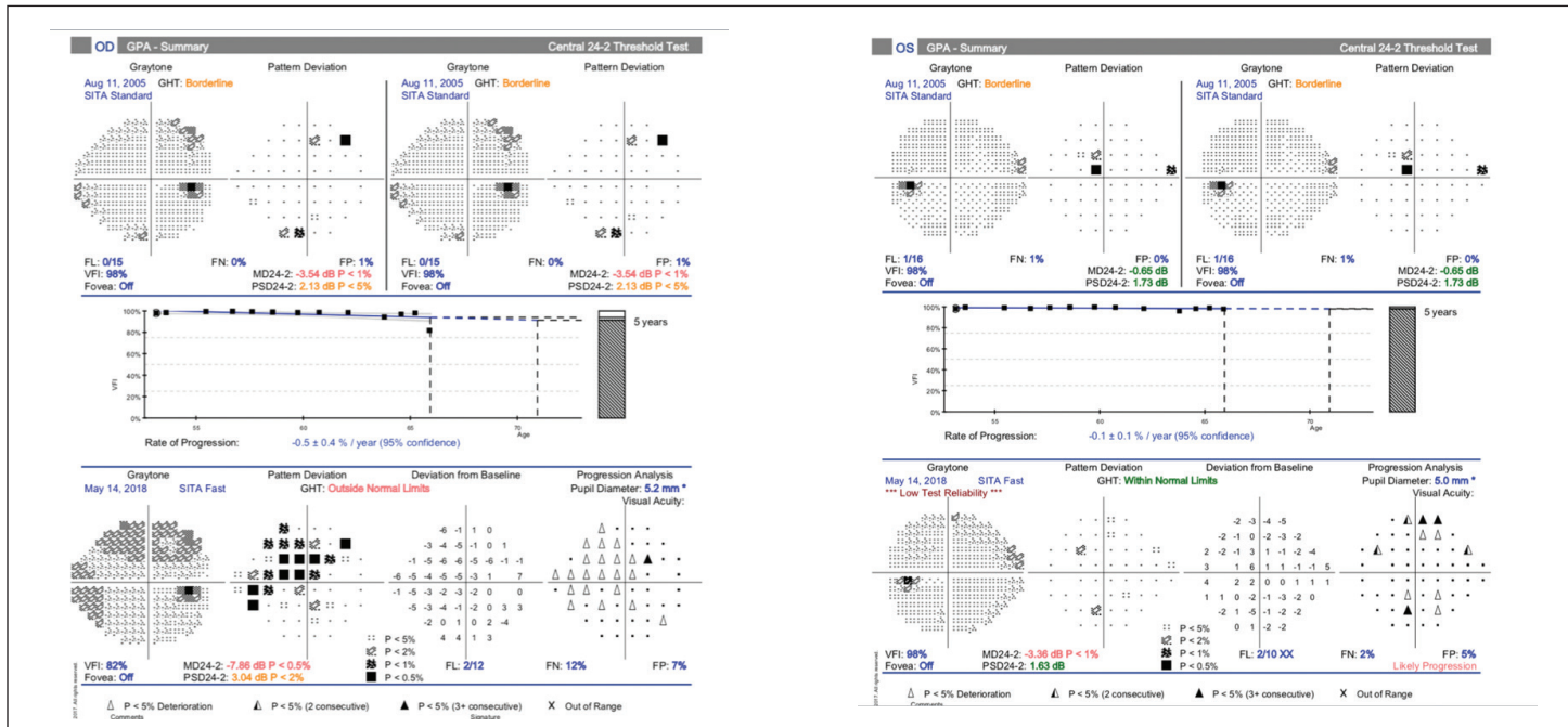
Figure 2. Seen here are the Humphrey GPA summary visual fields for the patient seen in Figure 1. The right eye has shown significant change with a superior arcuate visual field defect developing, requiring that the treatment regimen be modified. The change is also seen as the point on the Visual Field Index (VFI) trend line indicating the last exam has fallen below previous exam points. This case is illustrative of field defects showing up later in the course of glaucoma, with significant RNFL loss required.
